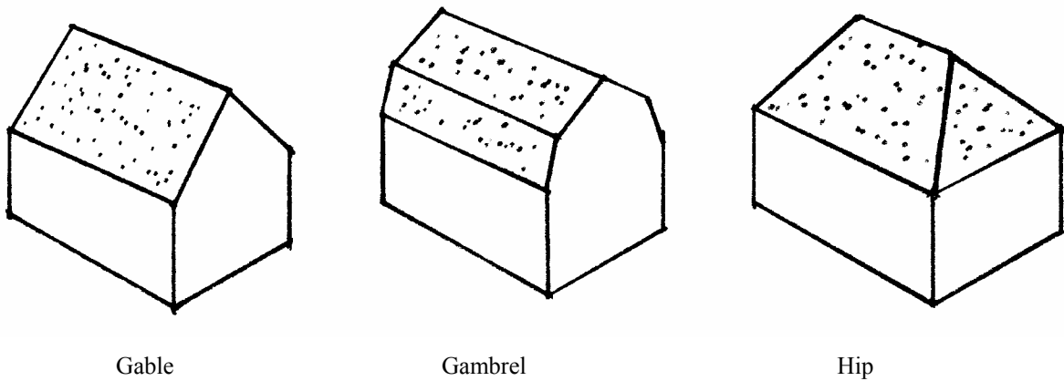
Figure 12. Roof Types
